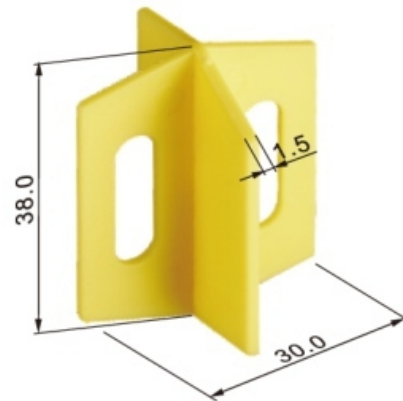
Multi-Function Spacer
