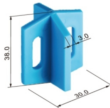
Multi-Function Spacer
